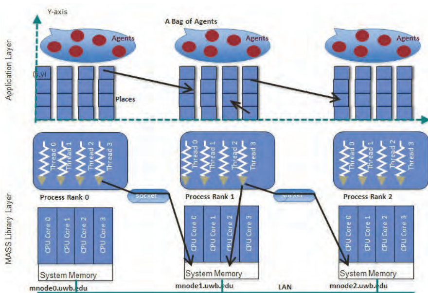
Figure 1: The MASS library's execution model
