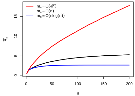
(b) Mean cumulative regret for the three regimes of the greedy policy over 500 macro replications.
