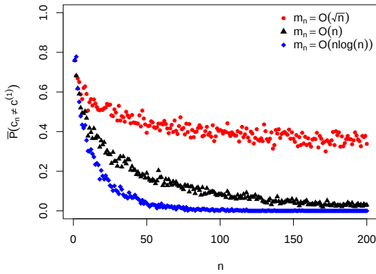
(a) Mean PICS for the three regimes of the greedy policy over 500 macro replications.
