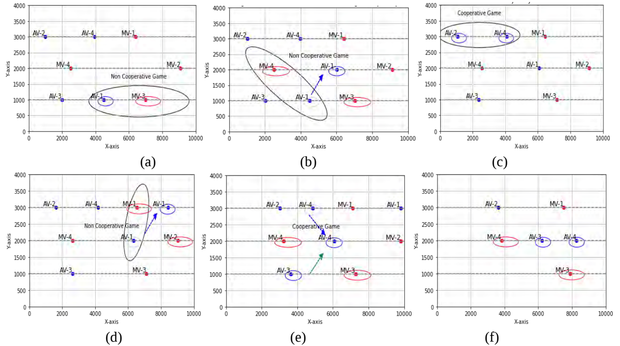
Figure 6: Simulation scenario 1: Collision avoidance analysis.
