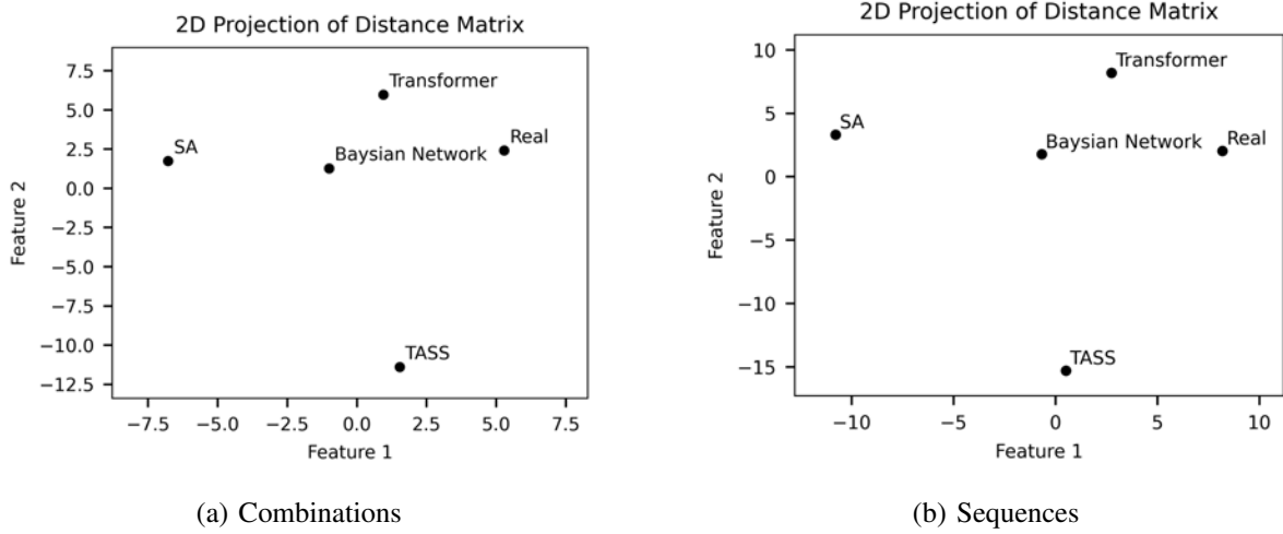
Figure 7: 2D projection of the resulting distance matrix between the weight matrices of the real-world dataset and the synthetic datasets using the Frobenius norm.
