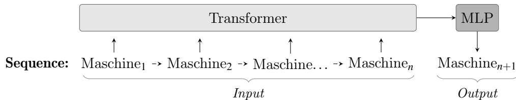
Figure 3: Simplified transformer architecture.
