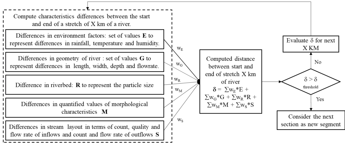
a) Algorithm to calculate number of river segments.
