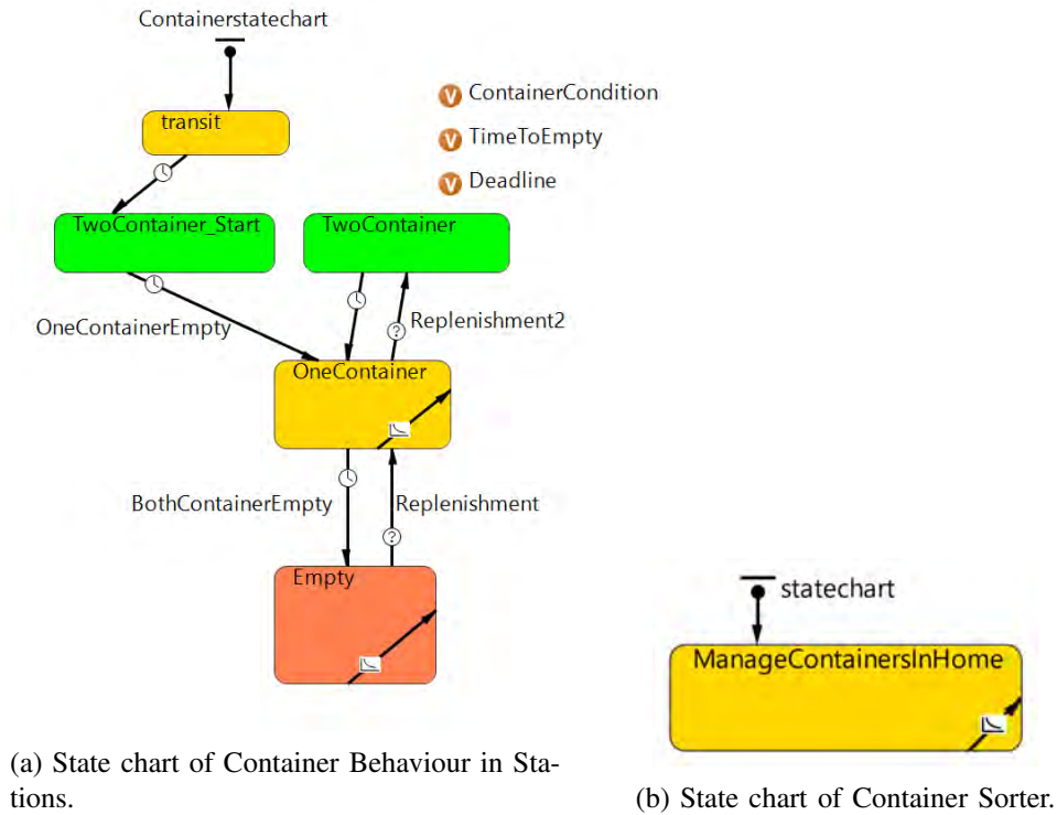
Figure 3: ABM parts for our model.
