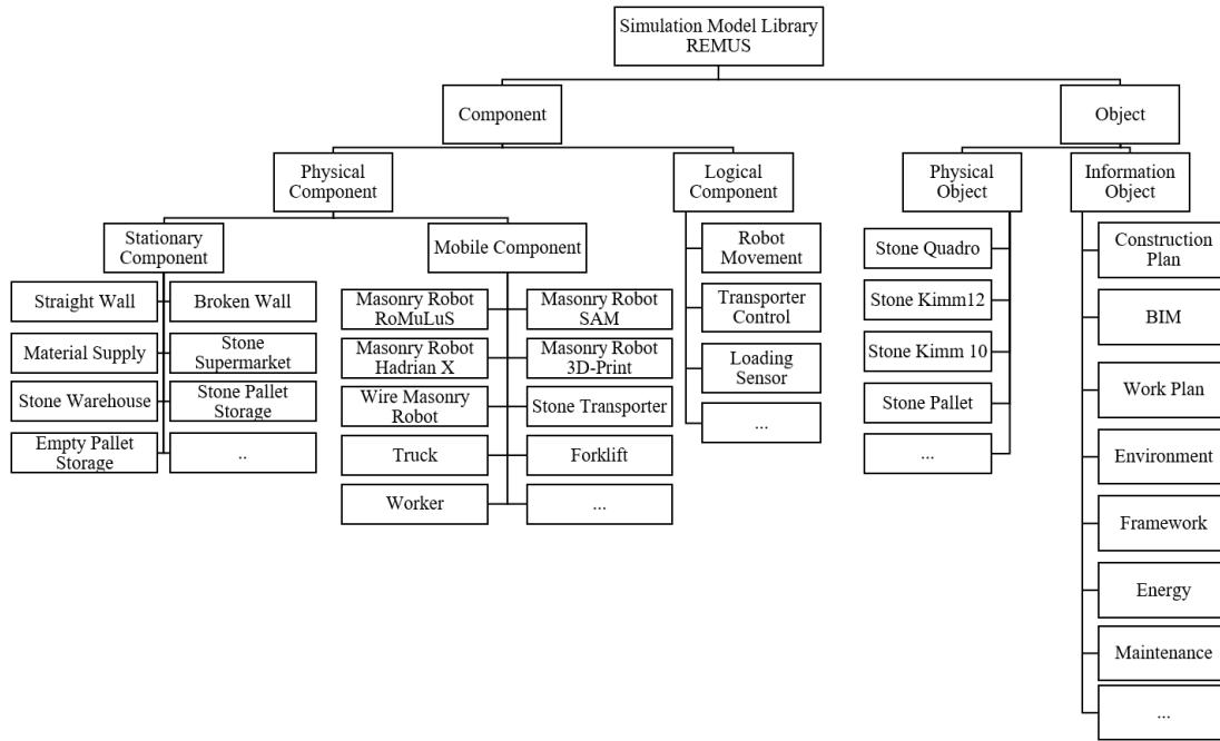
Figure 2: Simulation model library REMUS
