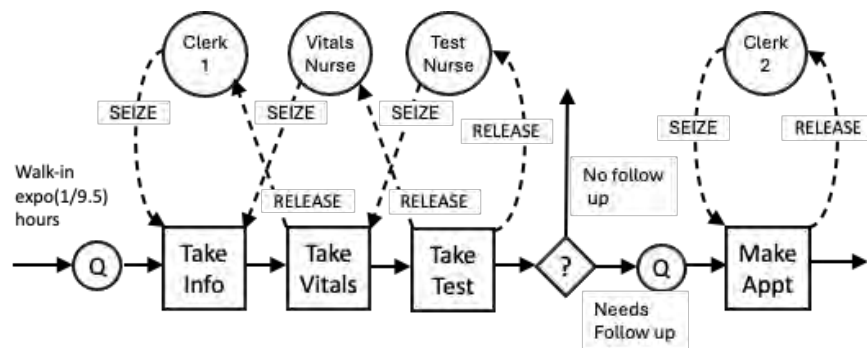
Figure 1: Activity Diagram for Design B Process
