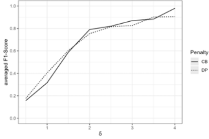
(a) Scaling signal-to-noise ratio via \delta and resulting F1-score for both penalty choice approaches.
