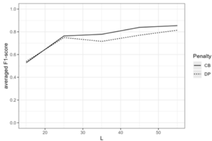
(a) Scaling signal-to-noise ratio via L and resulting F1-score for both penalty choice approaches.
