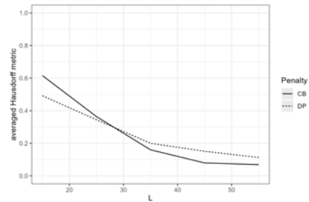
(b) Scaling signal-to-noise ratio via L and resulting Hausdorff metric for both penalty choice approaches.
