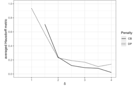
(b) Scaling signal-to-noise ratio via \delta and resulting Hausdorff metric for both penalty choice approaches.
