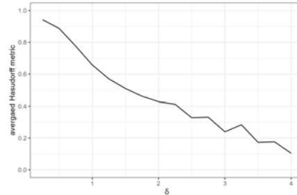
(b) Scaling signal-to-noise ratio via \delta and resulting Hausdorff metric.
