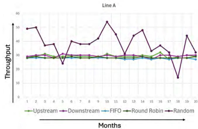
Figure 5: Line A throughput by policy (recorded every 30 days).
