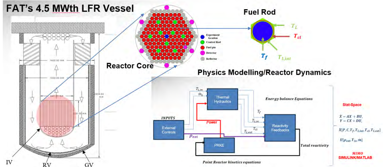
Figure 2: FAT's 4.5 MWth Reactor conceptual design, detailing the reactor core and schematic representation of the NTC coupling (blue rectangles).
