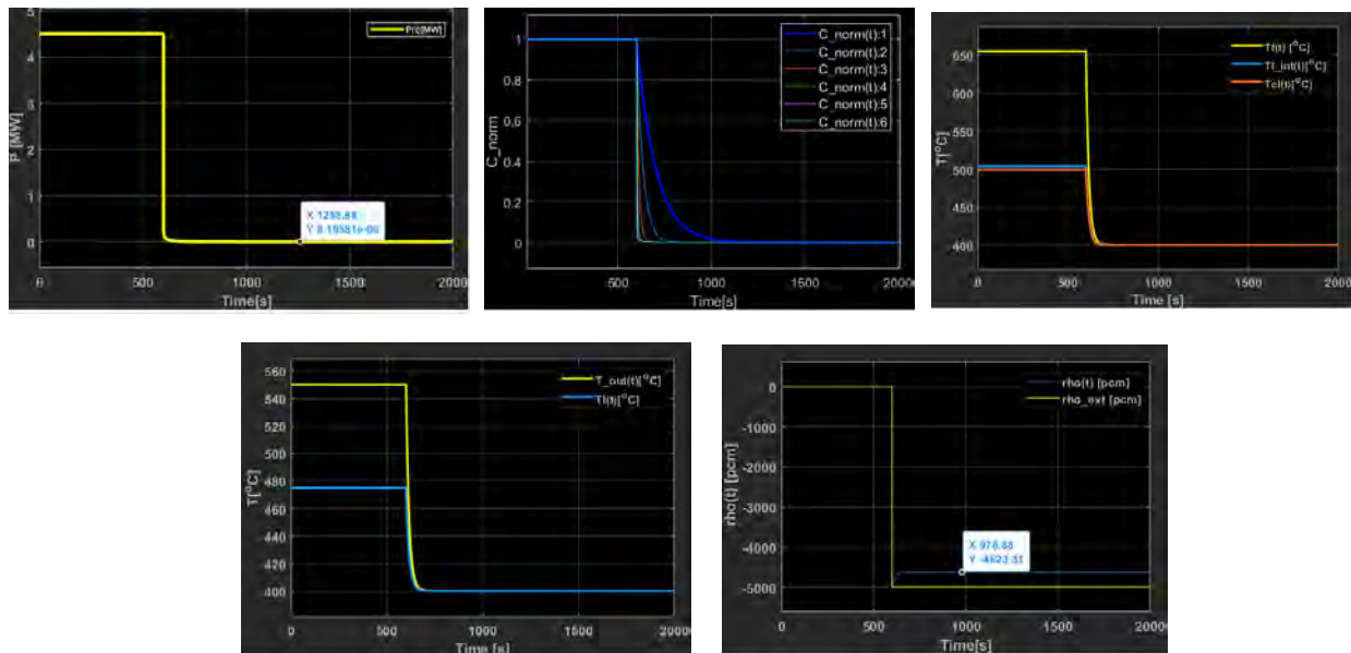
Figure 6: Reactor response to SCRAM; Power decays to zero and temperatures reduce to 400 °C.
