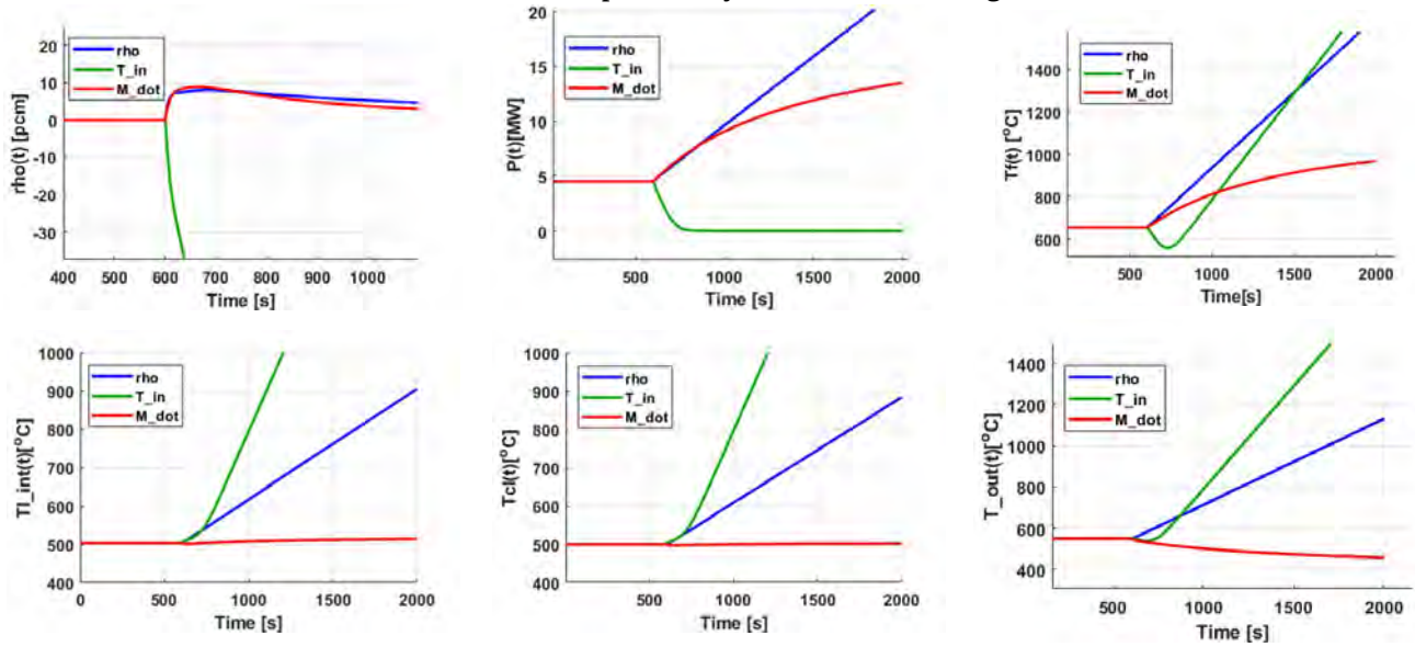
Figure 3: Reactor response from ramp inputs.
