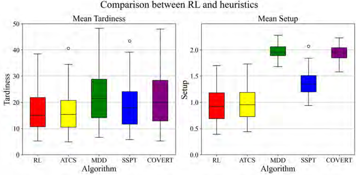
Figure 2: Mean tardiness and setup of RL and heuristics after 100 instances.
