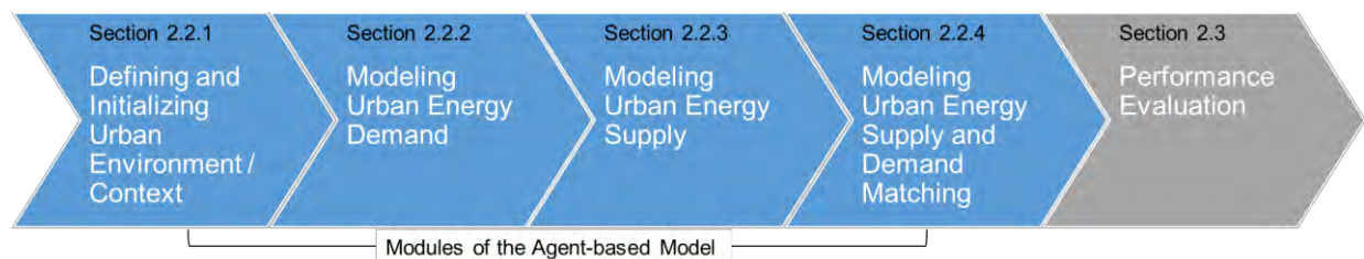
Figure 2: Methodology flowchart.
