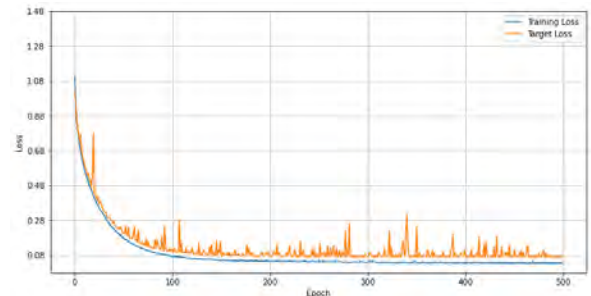
Figure 9: Loss curve - mobility network.
