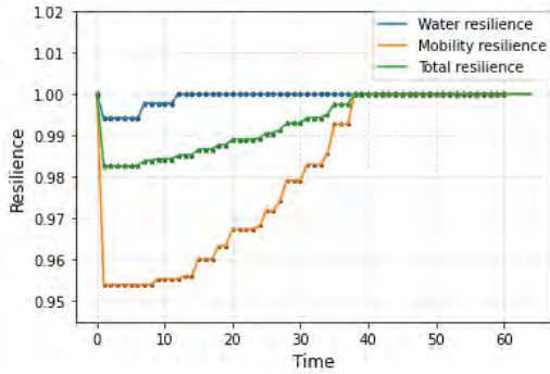
Figure 10: Network resilience over time - FIFO order.
