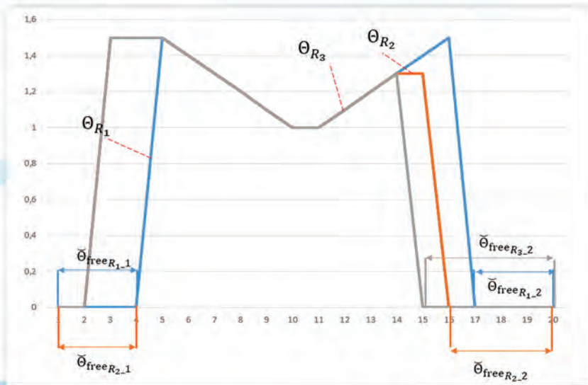
Fig. 4. Development of common visual field and regrouping decision making for UUV group
