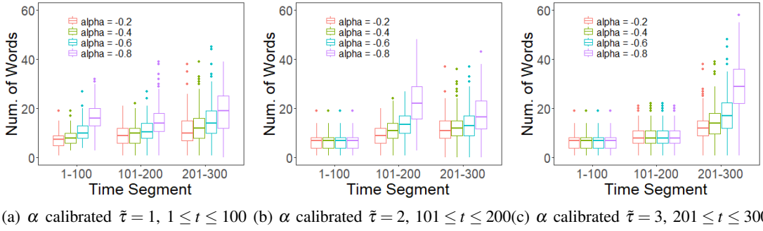
Figure 7: Number of words formed by all three agents in the graph for each \tilde{\tau} and each \alpha , when the VA is active in (a) \tilde{\tau} = 1 , (b) \tilde{\tau} = 2 , and (c) \tilde{\tau} = 3 . Each plot contains the average results from two simulations: one where VA is the hub node ( v_0 ) and one where the VA is a leaf node ( v_1 ). Each plot contains three collections of boxes, corresponding the cumulative number of words formed in each of the time ranges [1, 100] , [101, 200] , and [201, 300] . The four boxes in each collection correspond to the four values of \alpha . Results show that when a VA is active during one particular time segment, the effects continue, in the form of elevated numbers of words formed, in subsequent time segments.
