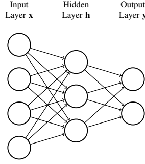
Figure 1: Multi-layer perceptron.
