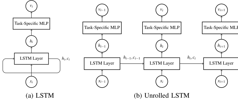
Figure 4: LSTM network.
