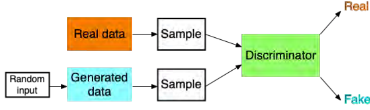
Figure 6: Generative adversarial network.
