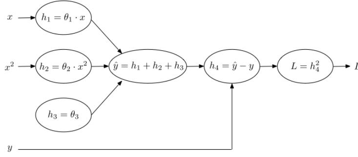
Figure 2: Stylized neural network for computing loss L .
