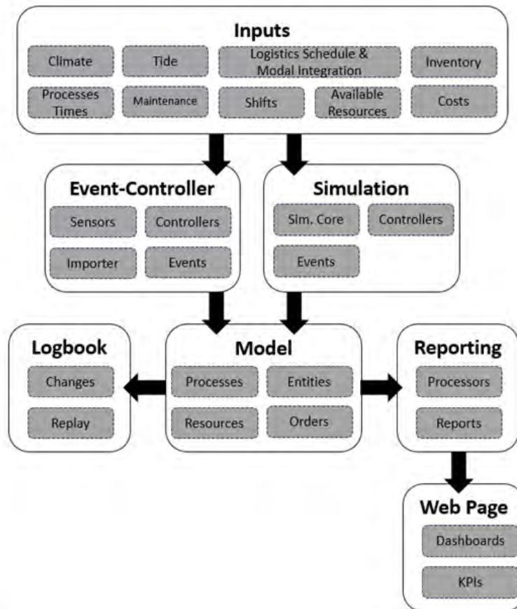
Figure 4: Architecture of the digital twin.
