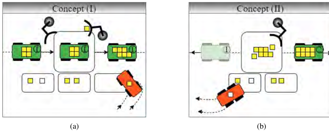
Figure 3: (a) Concept I: AGV staying at a workstation with a product, (b) Concept II: AGV leaving the workstation after unloading a product.
