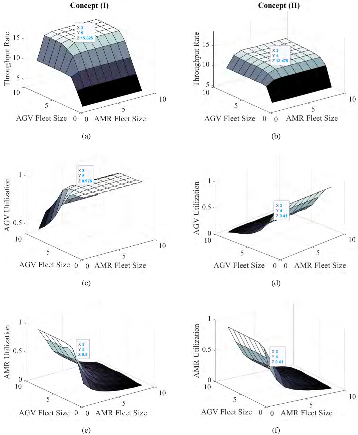
Figure 6: Hourly throughput rate (a) and (b), Average utilization of the AGV fleet (c) and (d), and Average utilization of the AMR fleet (e) and (f), under concepts (I) and (II), respectively.
