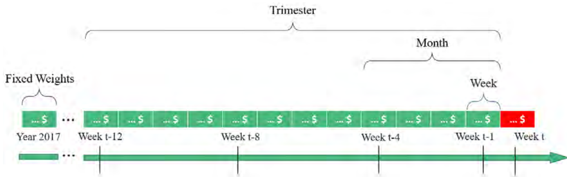
Figure 7: Parametrization methods
