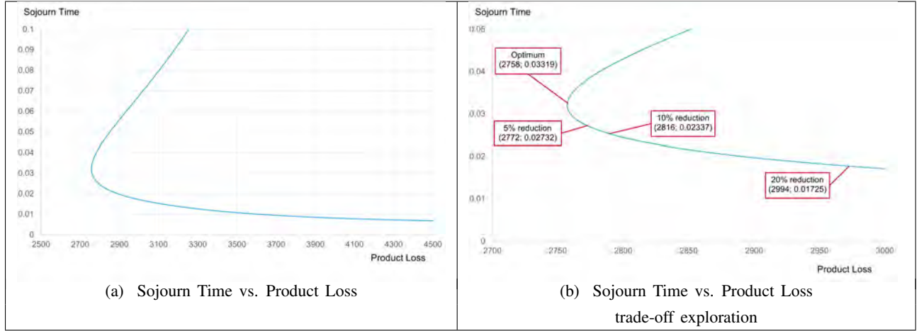
Figure 2: Sojourn Time vs. Product Loss for R = 10 ; p_{max} = 0.05 ; TP_{min} = 100 ; \frac{R \cdot \overline{TP}}{TM_r} = 30 ; v = 2
