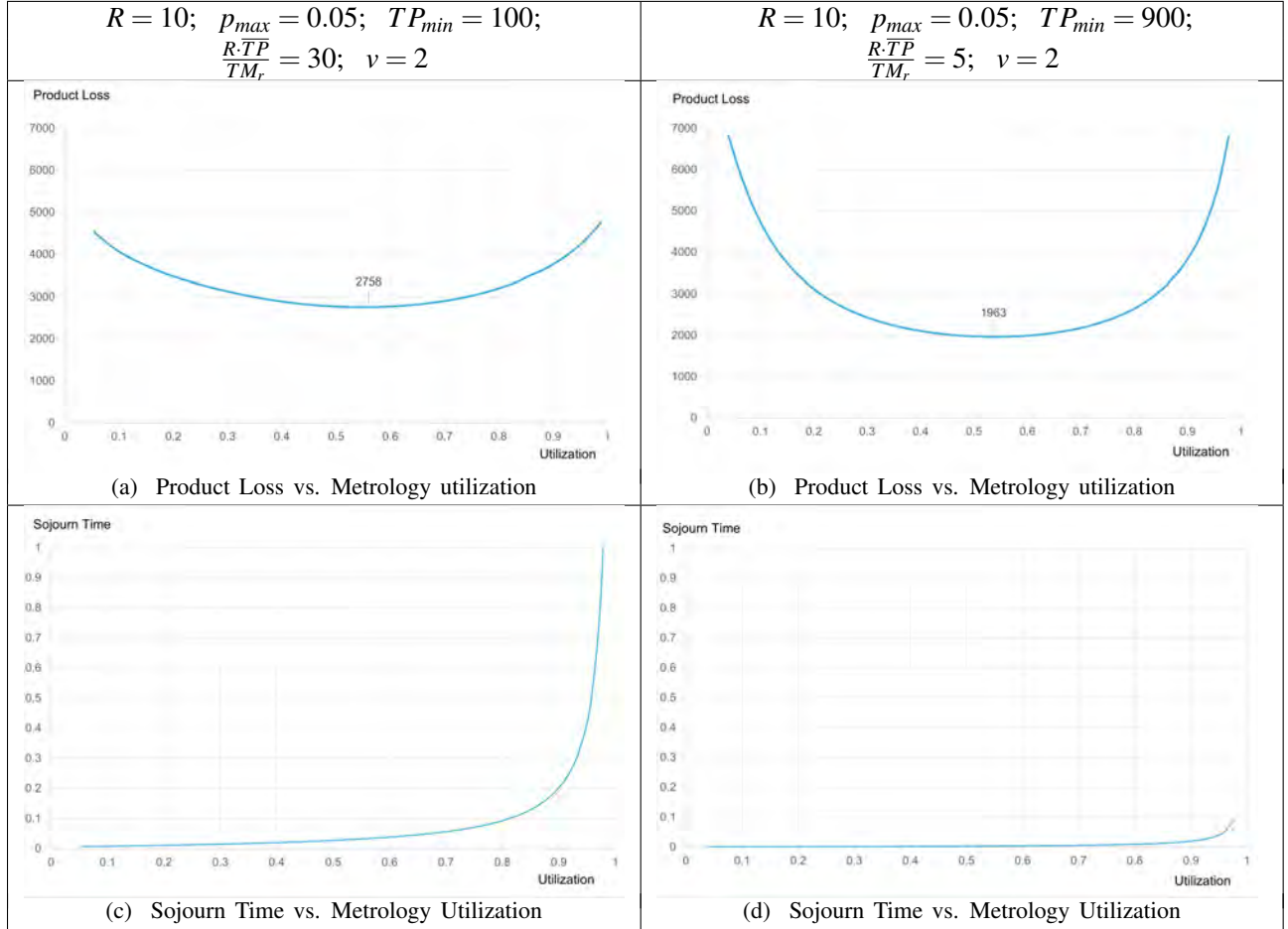
Figure 1: Product Loss vs. Metrology utilization and Sojourn Time vs. Metrology Utilization for two problem instances
