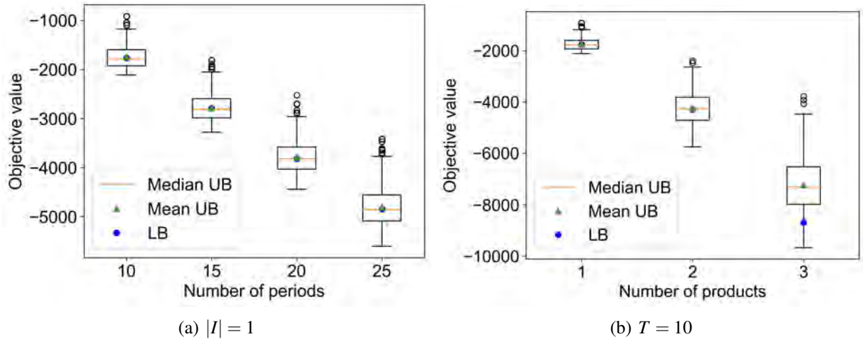
Figure 1: Box plots of the cost (objective function) incurred for n = 1000 simulations from Algorithm 2. The blue dots represent the lower bound, V_1^L(x_0, \omega_1) , calculated using Algorithm 1. The green triangles represent \hat{v} , the estimated expected cost calculated using n = 1000 sample path simulations. Part 1a shows results for T = 10, 15, 20, 25 periods for a family of single-product instances. Part 1b shows similar results for |I| = 1, 2, 3 products when T = 10 .
