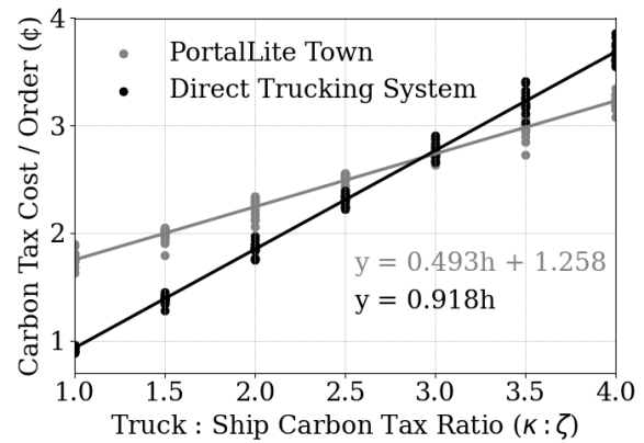
Figure 7: Emission ratio on carbon tax cost. The PortalLite systems reduces system emissions at \kappa/\zeta ratios of greater than 3.
