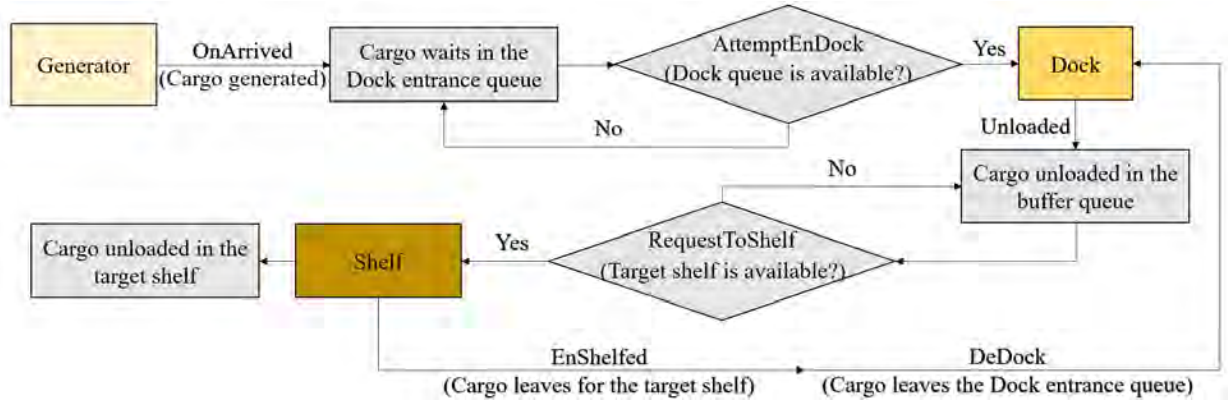
Figure 7: Illustration of warehouse simulation model.
