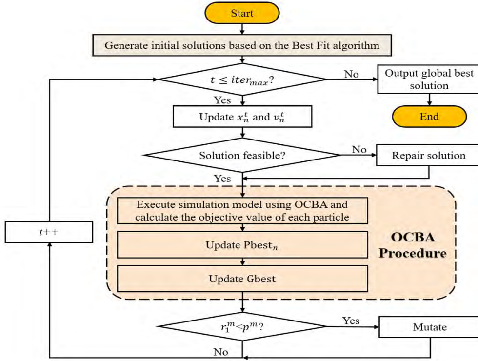
Figure 8: PSO-OCBA algorithm.
