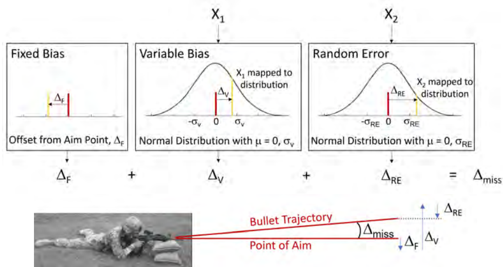
Figure 1: The miss angle ( \Delta_{miss} ) is the sum of the fixed bias ( \Delta_F ), variable bias ( \Delta_V ), and random error ( \Delta_{RE} ), which can be mathematically modeled from two random numbers fit into normal distributions.
