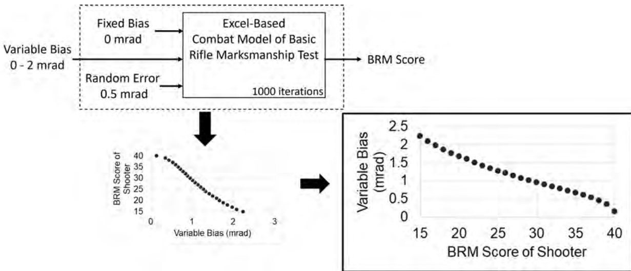
Figure 2: The methodology for determining the variable bias for a firer as a function of BRM score.
