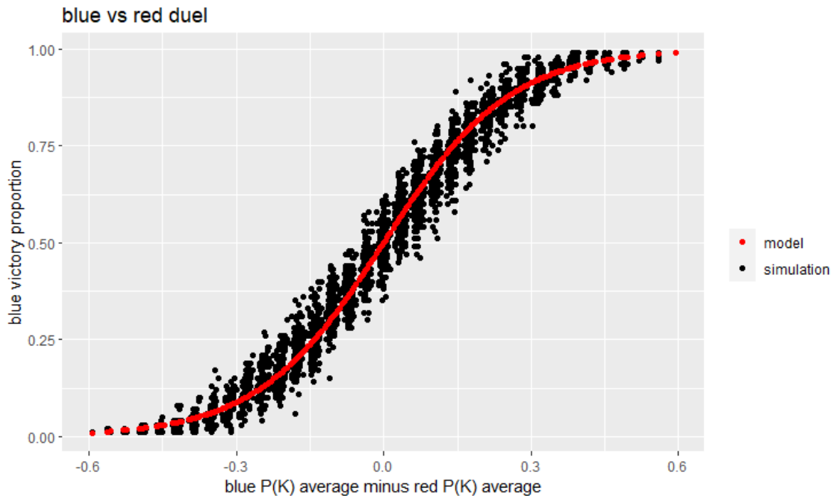
Figure 3: Results of simple stochastic duel where the marksmanship of each shooter was modified to look at changes in mission success.
