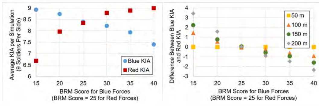
Figure 5: Average KIA for Blue and Red forces as a function of the Blue BRM score when the units are spaced 150 meters (left). Difference between the average Blue and Red KIA as a function of Blue BRM score when the units are spaced at different intervals (right).
