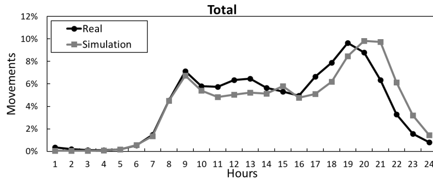
Figure 4: Comparison between the results of the Barcelona MATSim simulation against the real data provided in “EMEF” (see Table 1). The percentage of population that is travelling over the total is shown for each time bucket. Time bucket “1” covers from 00:00 until 00:59, bucket “2” covers from 01:00 until 01:59, and so on.
