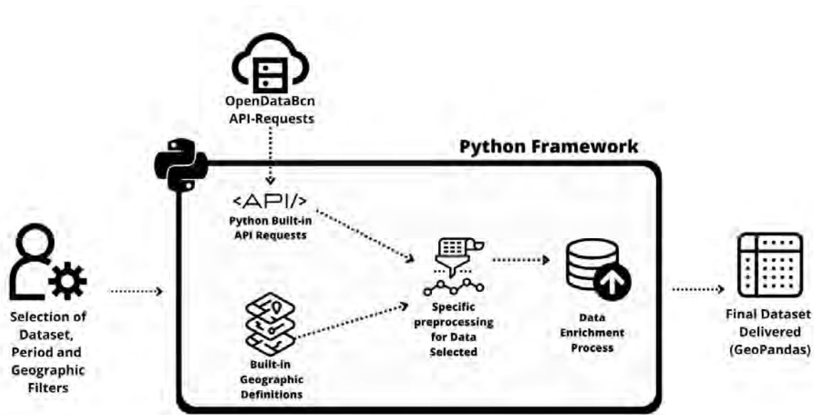
Figure 1: Preprocessing flow diagram designed for the use case.
