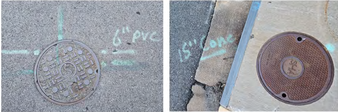
Figure 1: This is a field observation of the manual layout of construction utility. The left figure shows a 6" PVC pipe connected to a manhole. The right figure shows a 15" concrete pipe connected to a catch basin.
