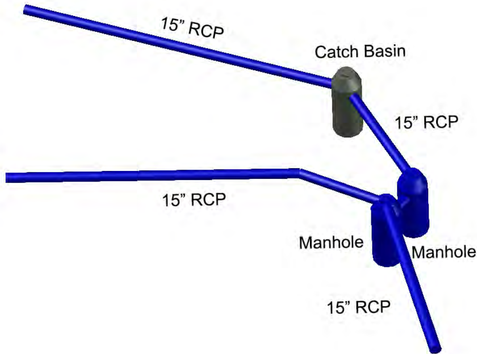
Figure 4: 3D model rendered in Civil 3D.
