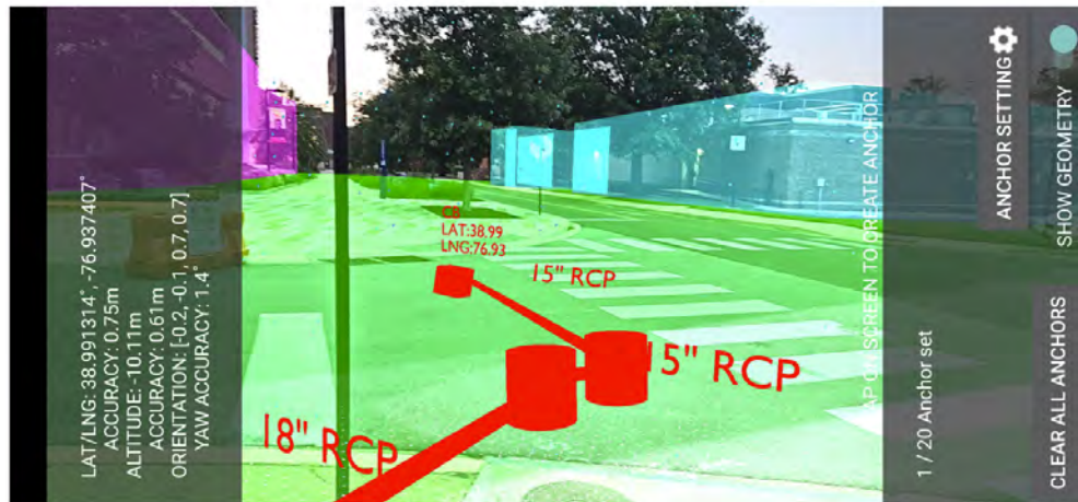
Figure 7: Superimposed utility layer with VPS recognized ground and building geometry on the real scene.
