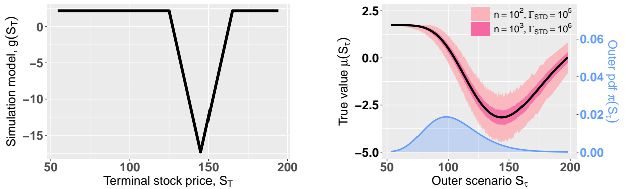
(a) Simulation logic g(S_T) for option portfolio example.
