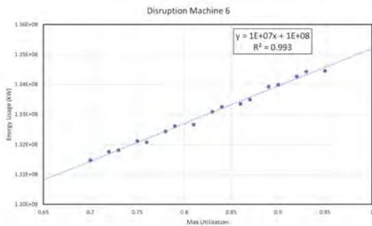
Figure 3: Energy usage and max utilization.
