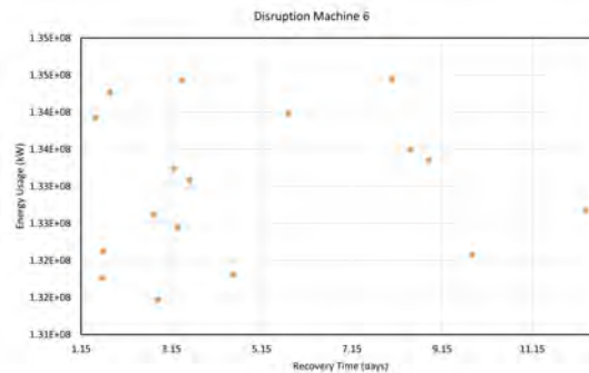
Figure 4: Energy usage and recovery time.
