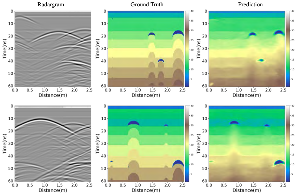
Figure 5: Example inversion results. The color bar value and the different colors indicate the dielectric constant values.
