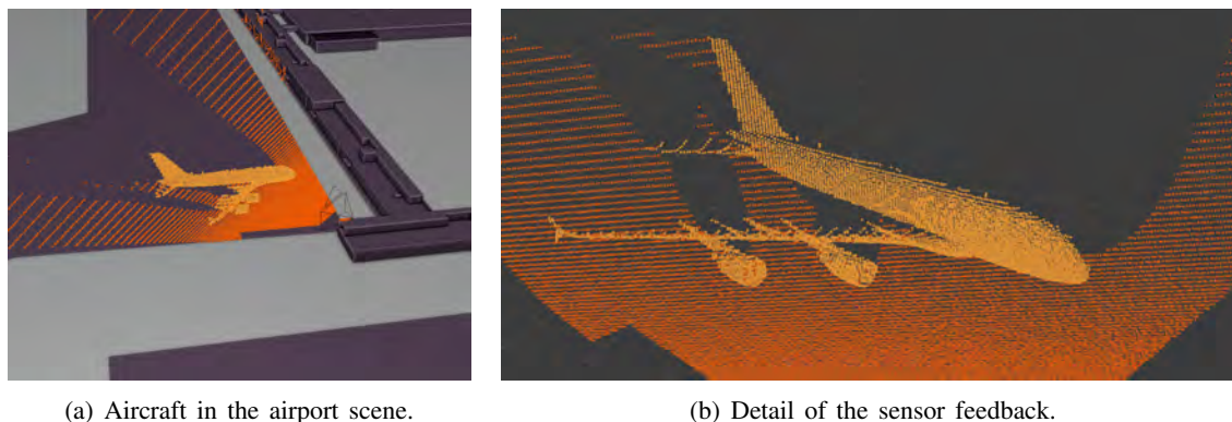
Figure 5: Synthetic LiDAR sensor feedback in the WSSS airport environment. With growing distance, the density of the emitted rays decreases.
