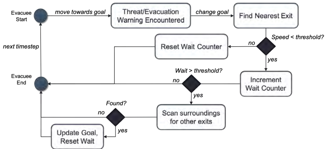
Figure 4: Panic Game Flowchart.
