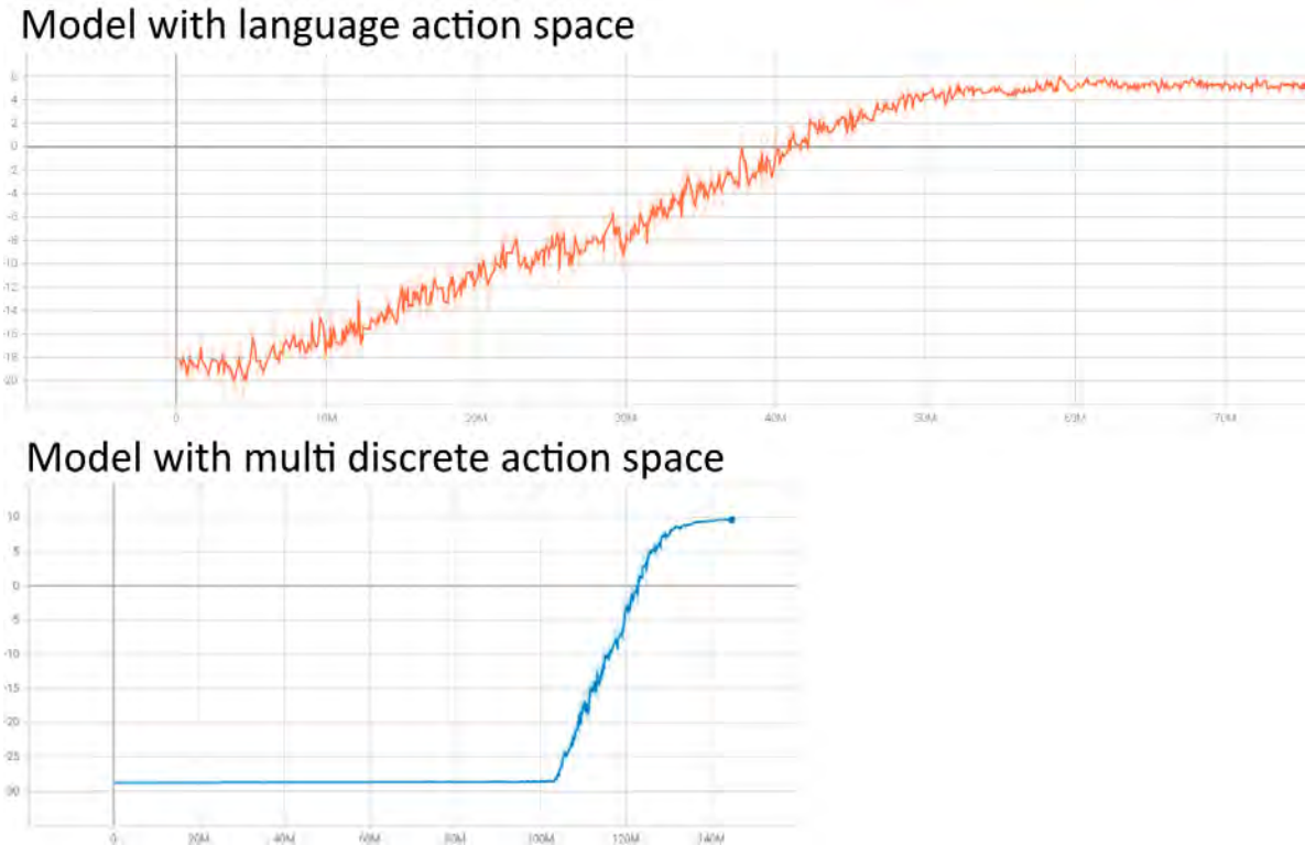
Figure 7: Action space comparison (language vs. multi-discrete action space).
