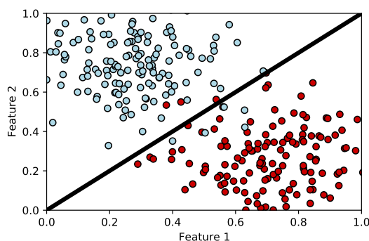
Figure 8: Binary classification in our case study. Due to the symmetric distribution of the two classes' features, an optimal linear separation of the classes is achieved by the diagonal (black line).
