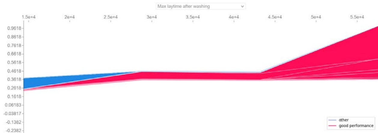
Figure 8: SHAP values plot for the factor maximum laytime after washing . The X-axis represents the factor value (in seconds), the y-axis represents the SHAP values.
