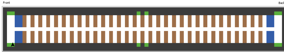
Figure 1: Example of boarding simulation for the Boeing 737 aircraft. Arrows correspond to passengers and their facing directions; white cells represent open spaces where passengers can walk freely, such as aisles and legroom; brown cells represent seats; blue cells represent aircraft internal structures; and green cells represent doors and emergency exits.
