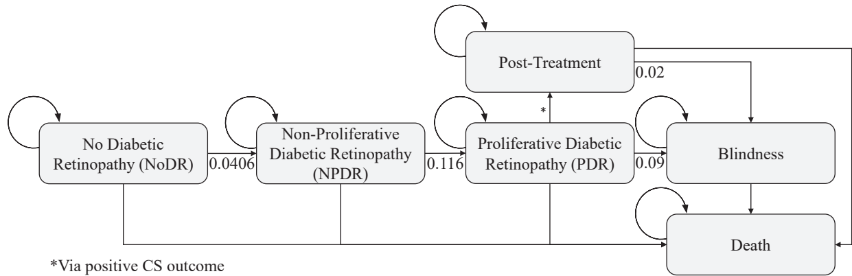
Figure 1: The Markov chain with all possible states and state transitions. Values on the arcs represent annual natural state transition probabilities for patients with 7% A1C. Death probabilities are defined by state and age-based mortality rates. Transitions to post-treatment occur only upon a positive CS.
