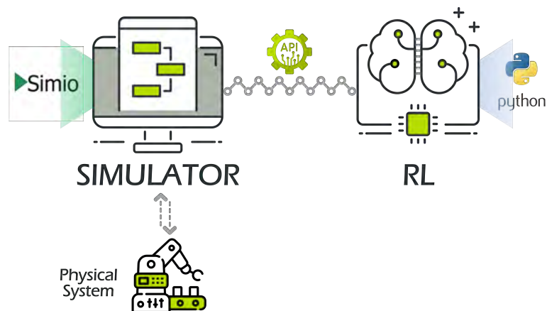
Figure 2: Simio-Python Integration.
