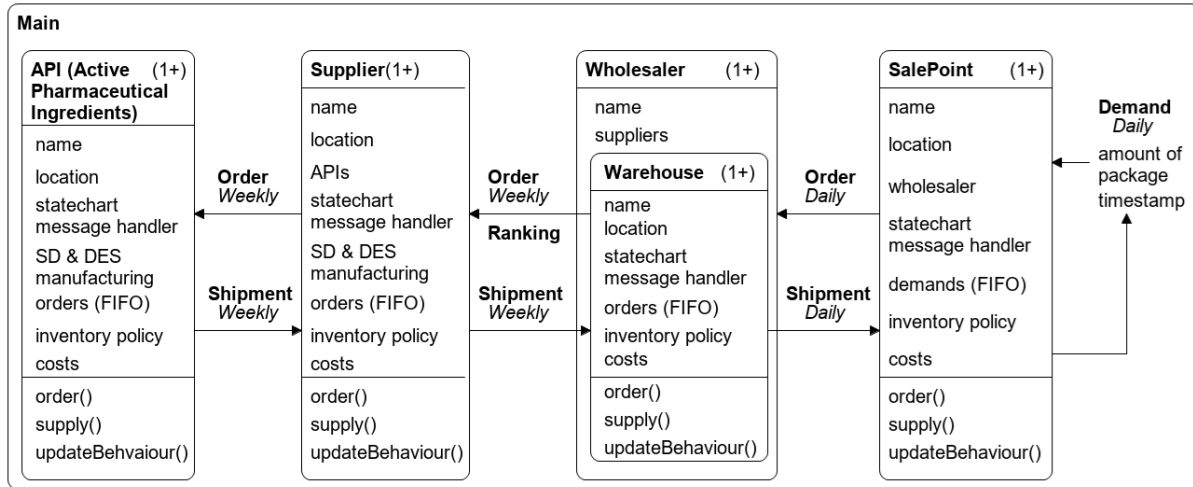
Figure 1: An overview of the HS modeling framework. Bold elements denote AnyLogic agents. High level variables and functions are stated. Queueing aspects of the model are signified by the First in First Out (FIFO) abbreviation. SD = System Dynamics. DES = Discrete Event Simulation.
