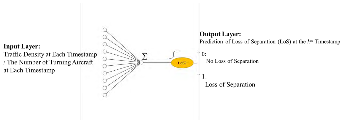
Figure 4: The structure of the Predicting Loss of Separation (LoS) method
