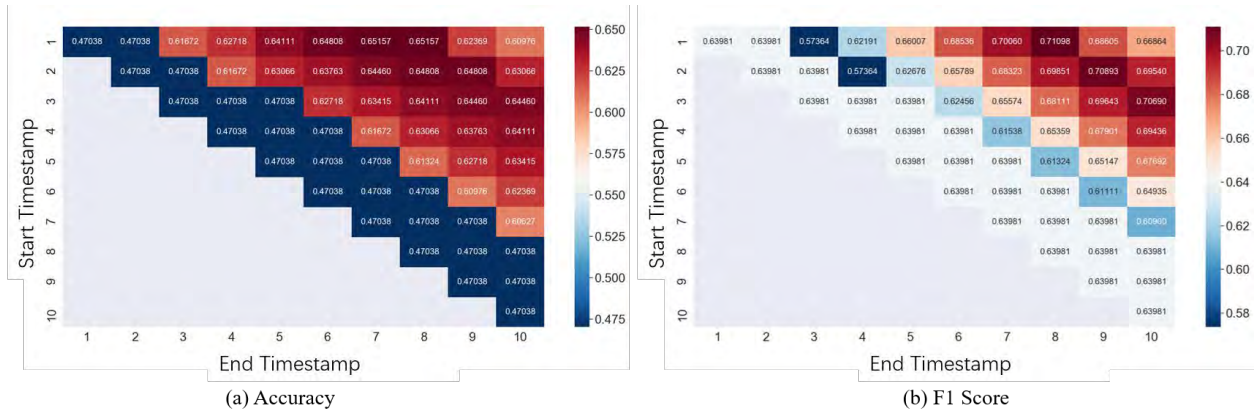
Figure 9: The accuracy and F1 Score in case 2 of scenario 2
