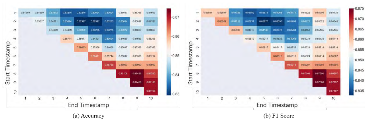
Figure 8: The accuracy and F1 Score in case 1 of scenario 2
