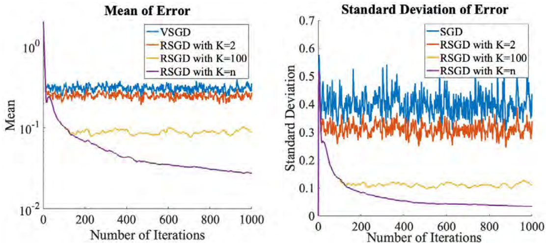
Figure 2: Mean and standard deviation of |\theta_n - \theta^*| of 100 runs of VSGD and RSGD with \alpha_n = 0.1, K = 2, 100, n .
