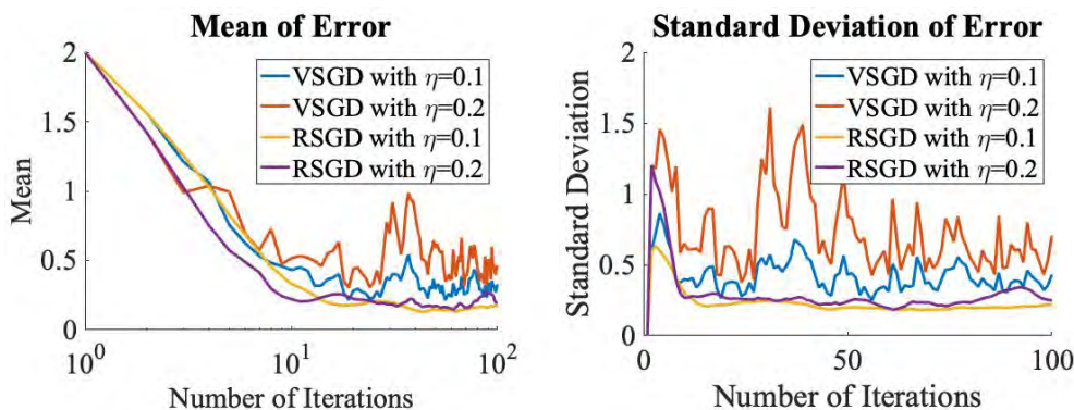
Figure 3: Mean and standard deviation of |\theta_n - \theta^*| of 100 runs of VSGD and RSGD with \alpha = 0.1, 0.2 .
