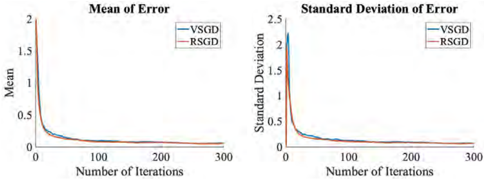
Figure 1: Mean and standard deviation of |\theta_n - \theta^*| of 100 runs of VSGD and RSGD with \alpha_n = \frac{1}{n}, K = 30 .
