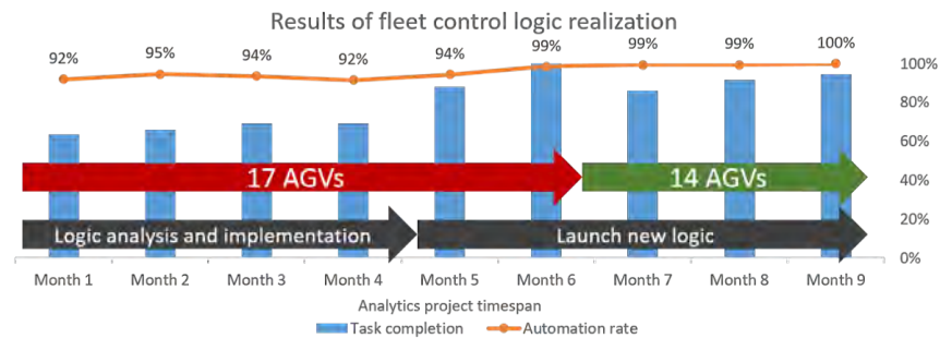
Figure 2: AGV system performance over the the time-span of the analytics project, with all results provided in percentages relative to the best value. Aside from the increase in the automation rate and the number of task completions, the new logic enables to maintain stable system operation with three vehicles less than previously.
