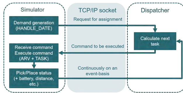
Figure 1: Architecture of the system's DES model, with the simulator and dispatcher sub-models and the TCP/IP socket communication between them.
