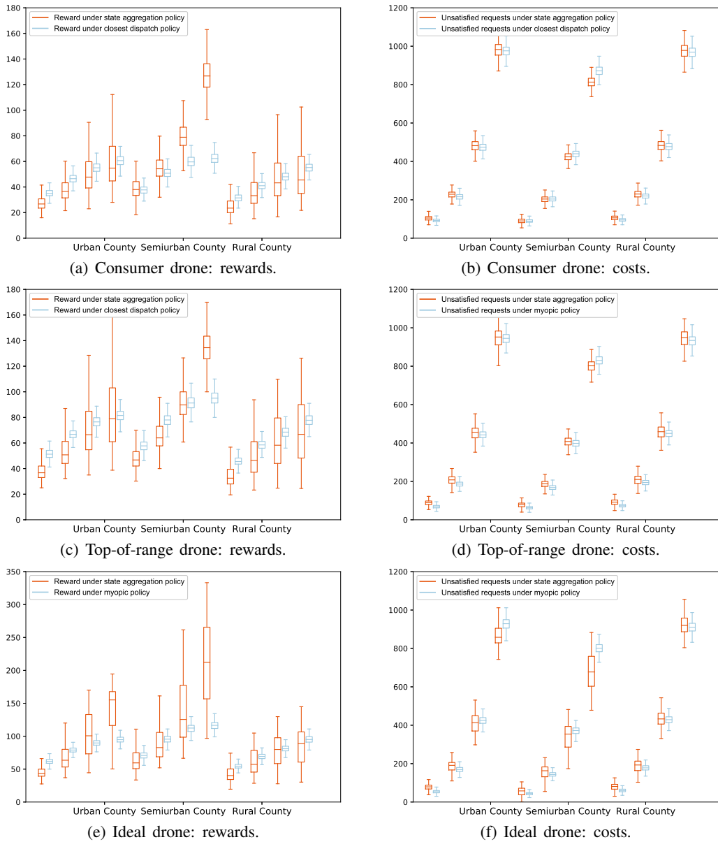
Figure 5: Performance comparison. For each UAV type, 12 settings are simulated for the overall arrival rate \lambda = 0.5, 1, 2, 4 and for the catchment area type being urban, semiurban, and rural (from left to right) and the results are presented in the two subfigures in each row.
