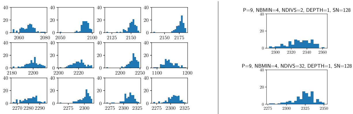
Figure 4: Histograms of observed throughputs when running HPL on four nodes with N = 20,000 , NB = 128 . The throughput distributions for the 12 highest mean throughput configurations are from Table 4 (left) and the two nondominated configurations are from Table 5 (right).
