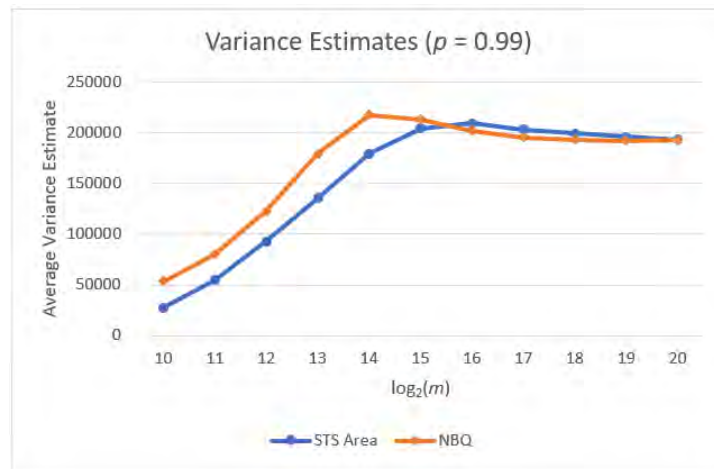
Figure 2: Average variance estimates for the marginal 0.99-quantile of a stationary waiting-time process in an M/M/1 queueing system with traffic intensity \rho = 0.8 . All estimates are based on 2500 independent replications with b = 32 batches and batch sizes m = 2^\ell , \ell = 10, 11, \dots, 20 .
