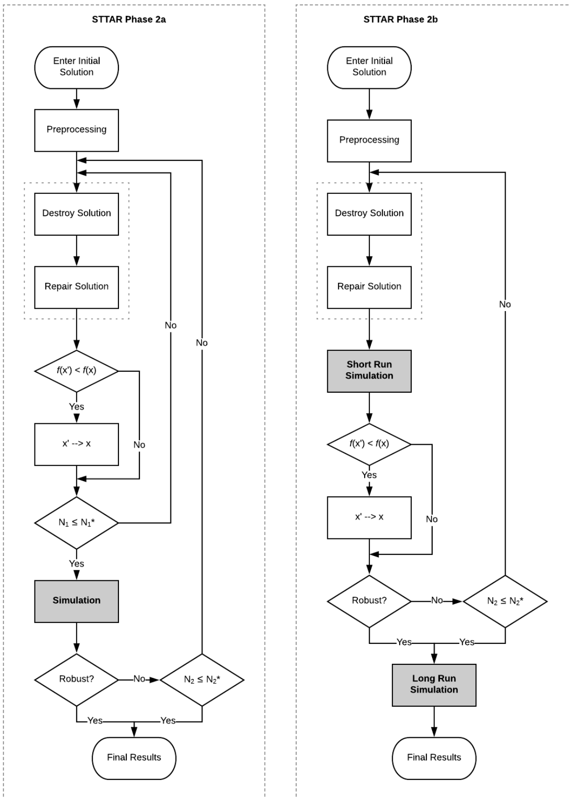
Figure 2: Simheuristic approach proposed for Phase 2 of STTAR.
