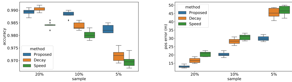
Figure 11: Comparison of accuracy and error in jam-tail position using proposed method, decaying average speed, and simple speed method with sample percentages.
