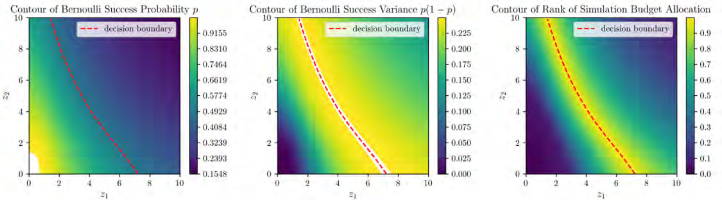
Figure 1: Demonstration of OCBA for Binary Classification with Unknown Structures.
