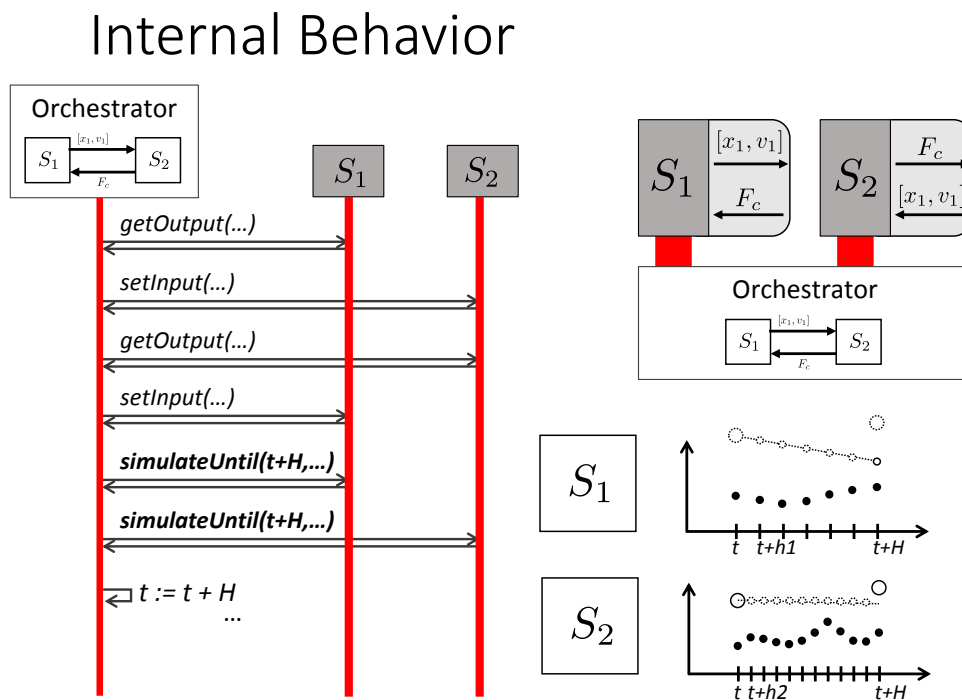
Figure 2: Example co-simulation coordination (left), co-simulation scenario (top right), and internal behavior of simulation units (bottom right).
